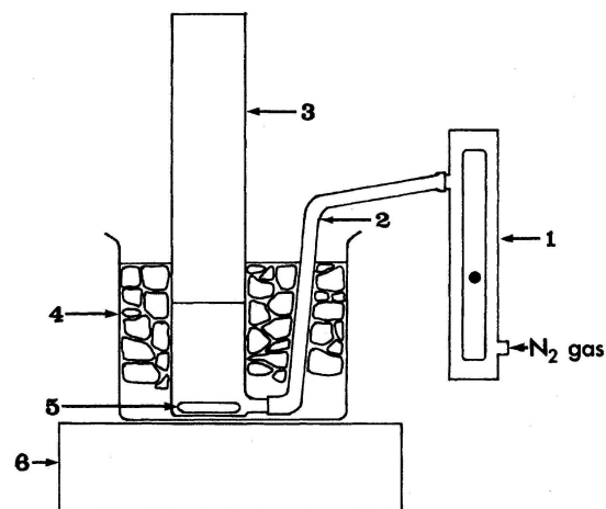
Fig. 1. Extraction apparatus for hydrogen peroxide 1, flow meter; 2, silicone tubing, 5mm id; 3, amber test tube, 25mm id × 180 mm; 4, ice-water bath; 5, magnetic stirring bar, 6 mm id × 20 mm; 6, magnetic stirrer.
